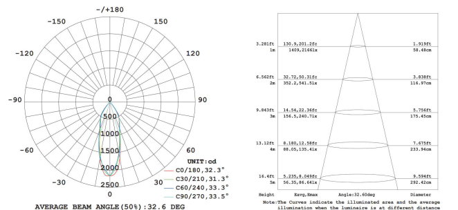
(12W luminous intensity and lux distribution diagrams)
